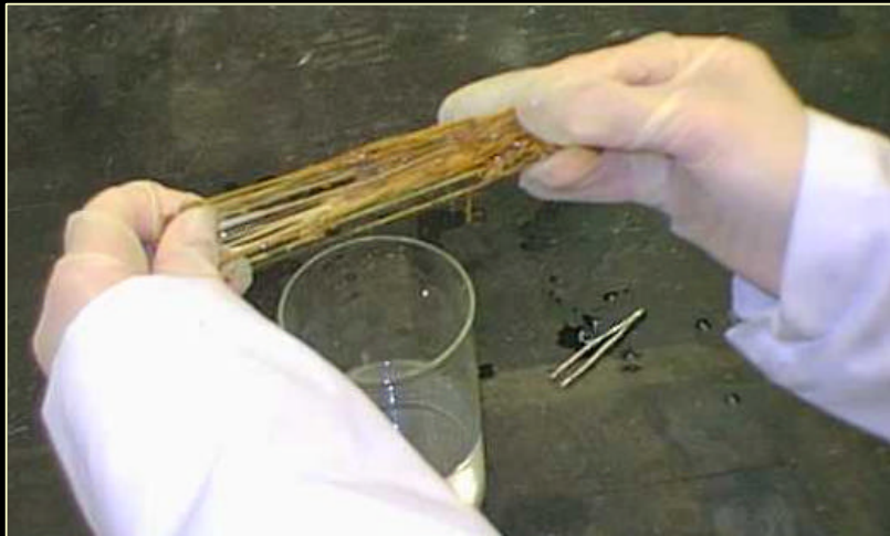
Amorphous Sulfur
